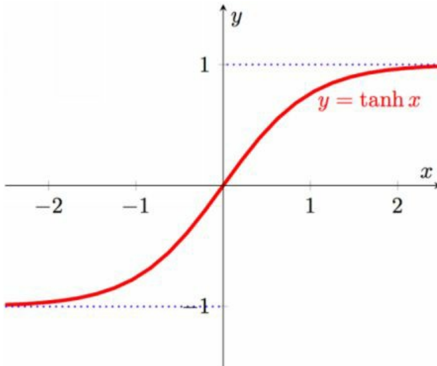
Figure 10: A hyperbolic tangent function graph
