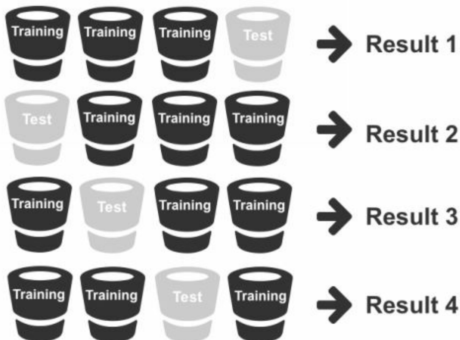
Figure 2: k -fold validation
